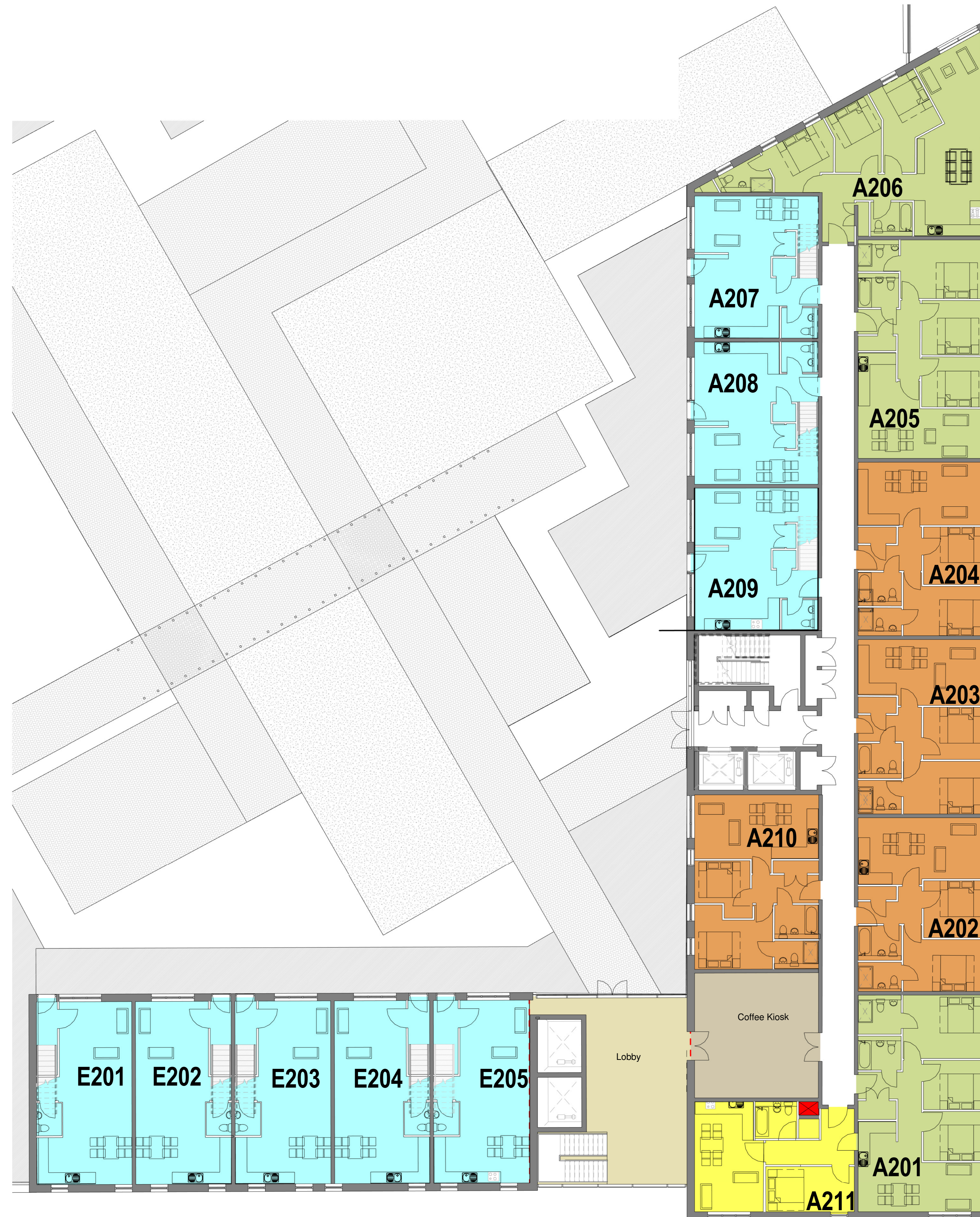
1 Blocks A & E - Second Floor 1:100
